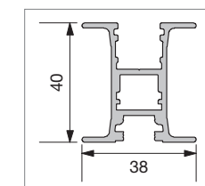
Griffprofil BASIC
